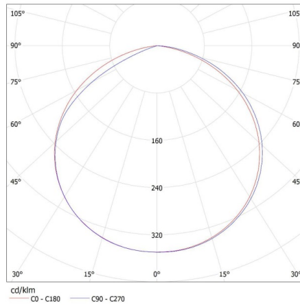
KANLUX S.A. (kat 33318) L48 9W_M 24 IP00-RGBW / LDC (Polar) Luminaire: KANLUX S.A. (kat 33318) L48 9W_M 24 IP00-RGBW Lamps: 1 x L48 9W_M 24 IP00-W
