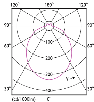
LEDspots Corepro SLR 1 4,9W PAR16 GU10 830 120D-LDD
